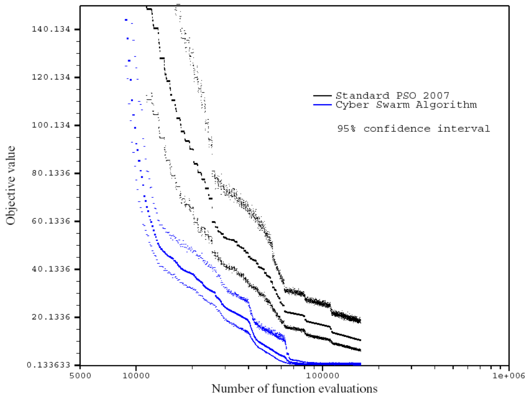
Fig. 4. The evolution of the best objective function value of the two competing methods with 95% confidence interval.
