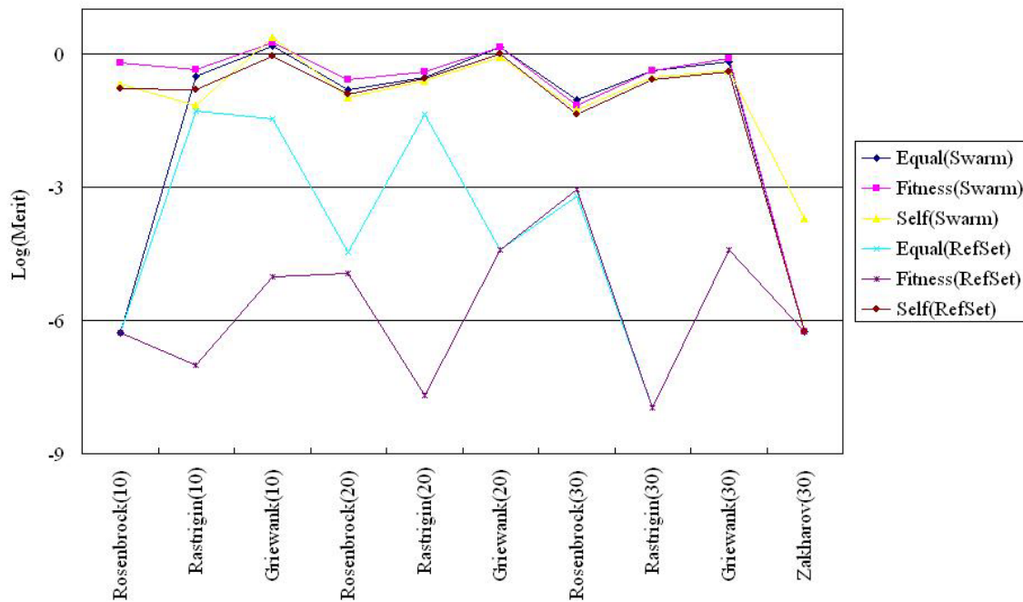
Fig. 8. Logarithmic value of the merit obtained using the best Cyber Swarm Algorithms with various weighting schemes.
