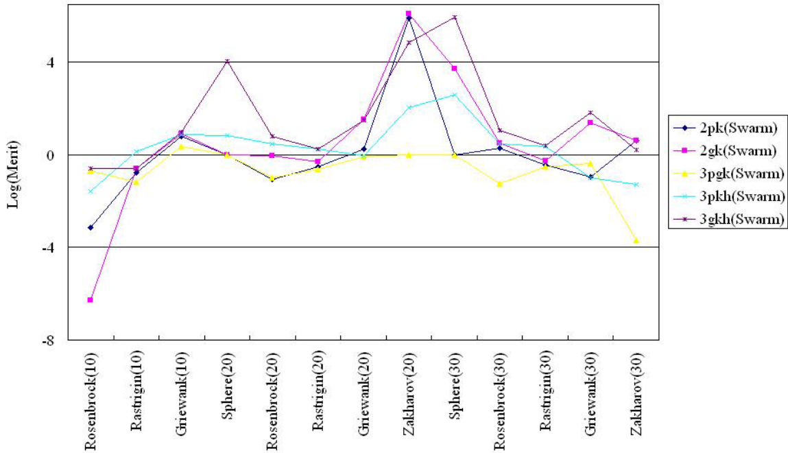
Fig. 6. Logarithmic value of the merit obtained using the Cyber Swarm Algorithms learning from swarm members.
