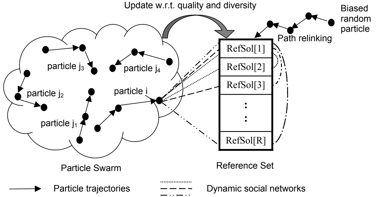
Fig. 2. Conception of the Cyber Swarm Algorithm.
