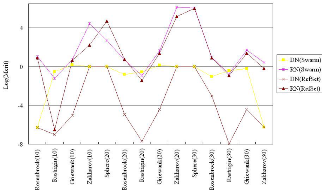
Fig. 9. Logarithmic value of the merit obtained using different forms of social network.
