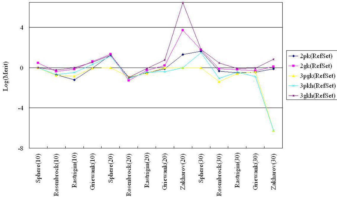
Fig. 7. Logarithmic value of the merit obtained using the Cyber Swarm Algorithms learning from RefSet members.
