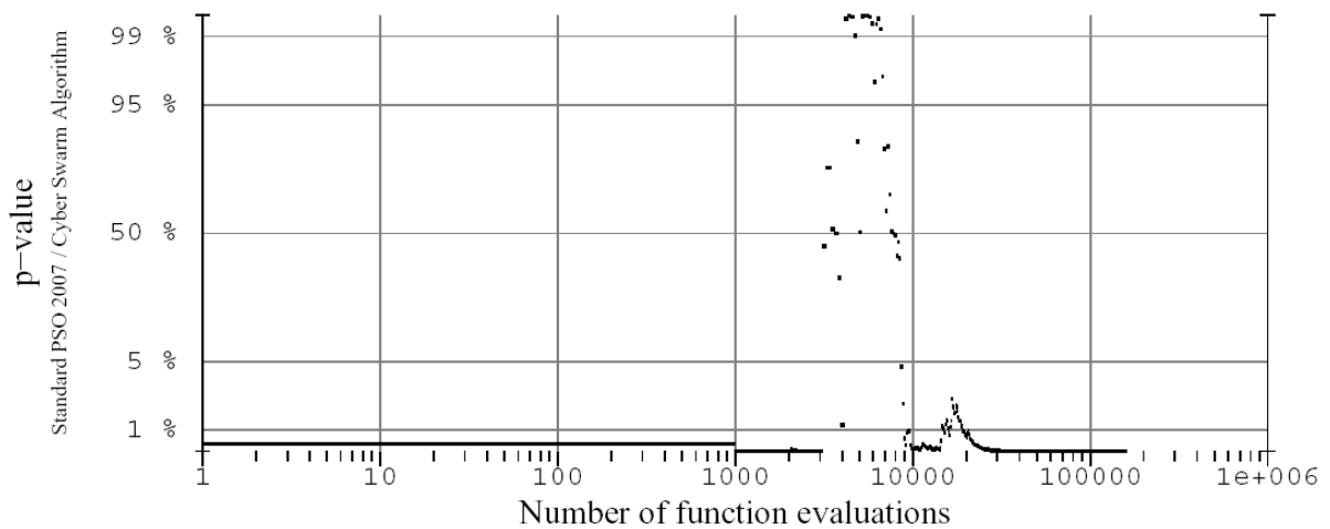
Fig. 5. The p -value for the Standard PSO 2007 being better than the Cyber Swarm Algorithm.
